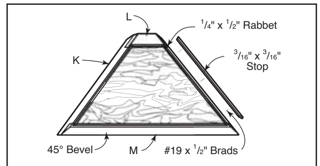
FIG 7B. INSIDE OF SHADE FRAME
