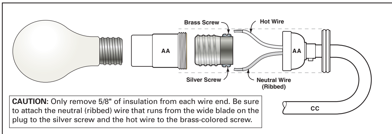
FIG 14. SOCKET ASSEMBLY
