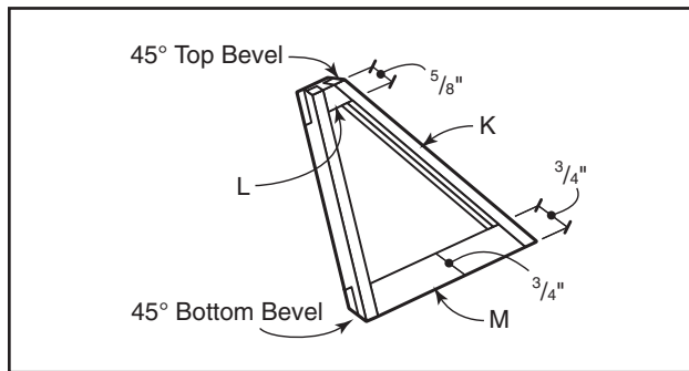
FIG 7A. BEVELED ENDS
