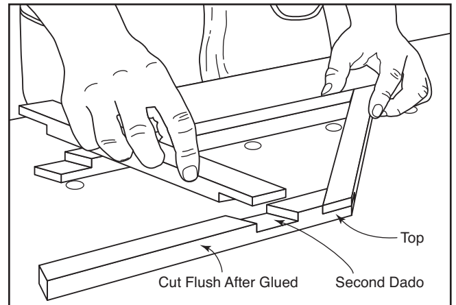
FIG 4. ASSEMBLE THE FRAME
