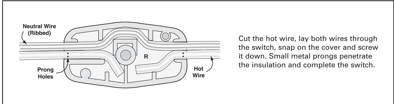
FIG 15. ROTARY SWITCH
