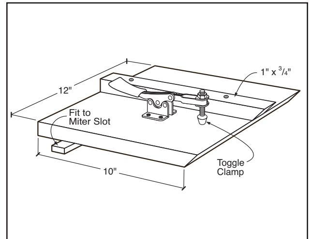
FIG 11. SPLINE SLOT SLED
