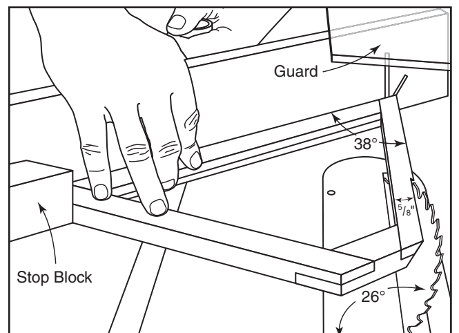
FIG 6. RIP THE COMPOUND ANGLES
