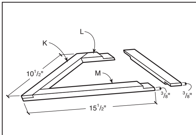
FIG 3. HALF-LAP JOINTS
