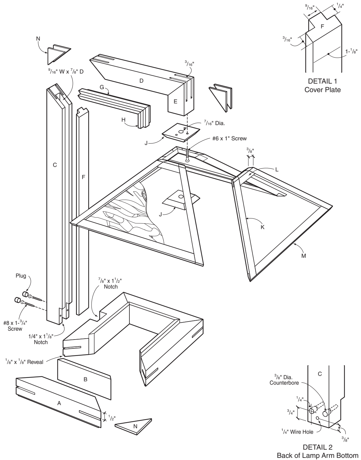
FIG 1. LAMP DETAILS
