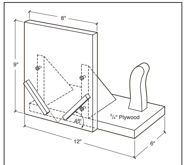
FIG 11. SPLINE SLOT SLED
