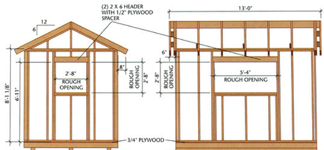
BUILDING SECTION
